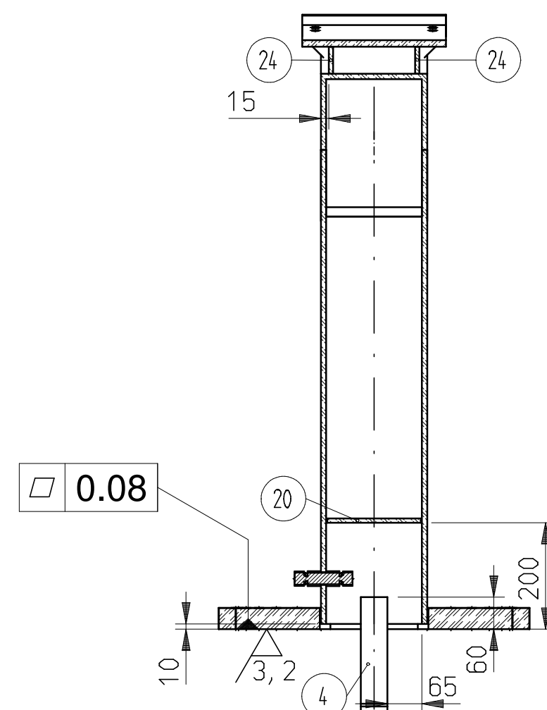
Cross-section B-B
